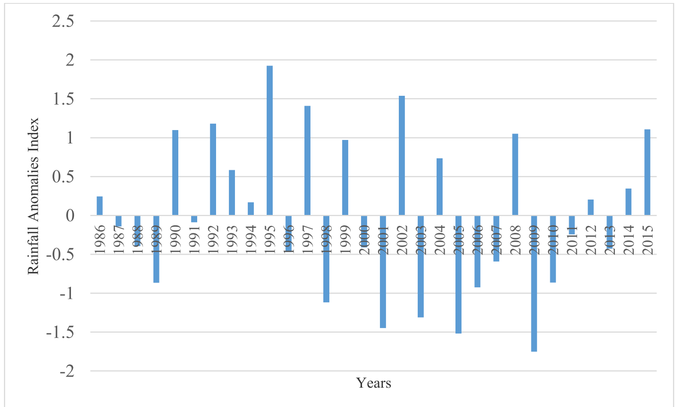
Figure 5: Pattern of Rainfall Anomalies in Warri, 1986-2015
