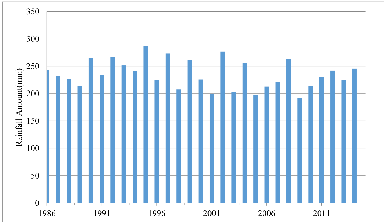
Figure 2: Mean Annual Rainfall (mm) in Warri, 1986-2015
