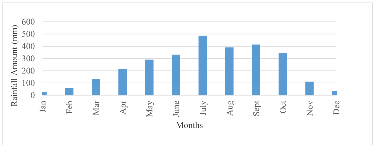
Figure 1: Mean Monthly Rainfall in Warri, 1986-2015
