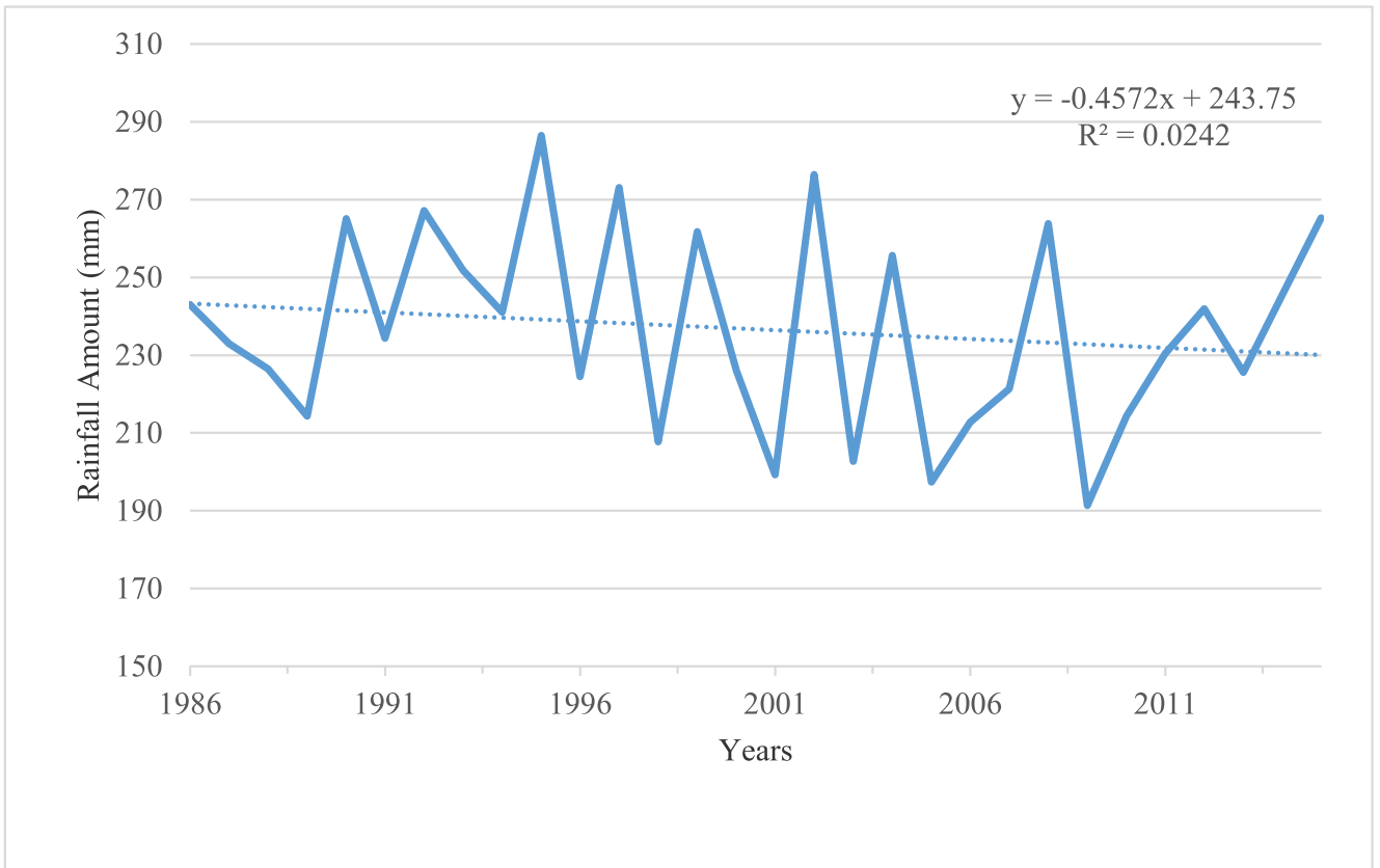
Figure 3: Rainfall Trend Pattern in Warri (1986-2015)
